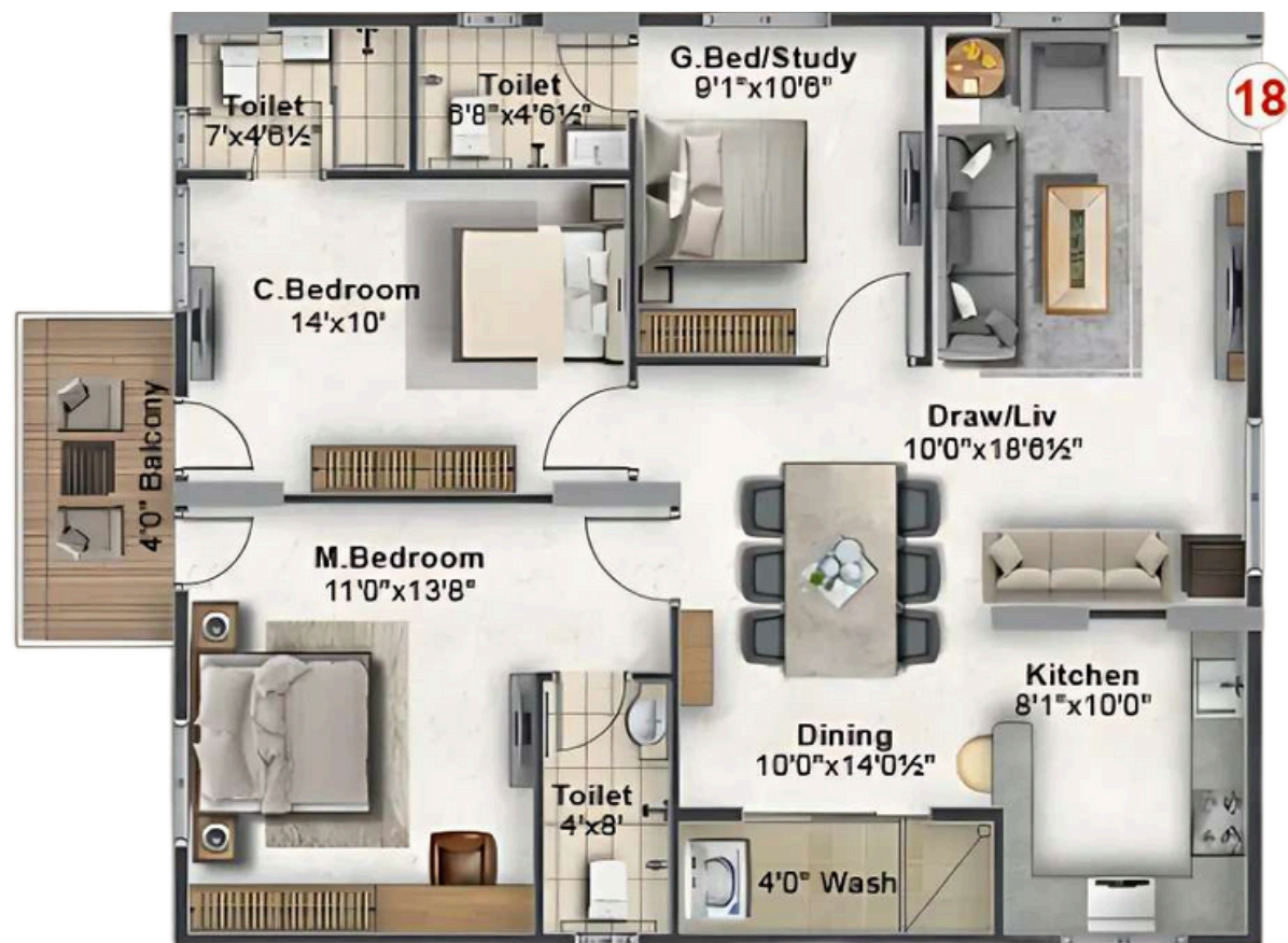
FLOOR PLAN EAST-FACING - FLAT NO.18 3 BHK 1350 SFT.
