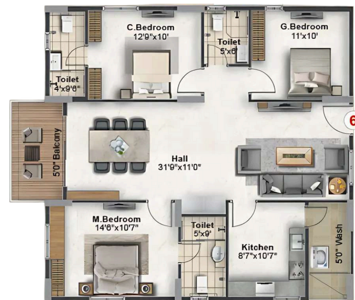
FLOOR PLAN WEST-FACING - FLAT NO. 6 3 BHK 1500 SFT.
